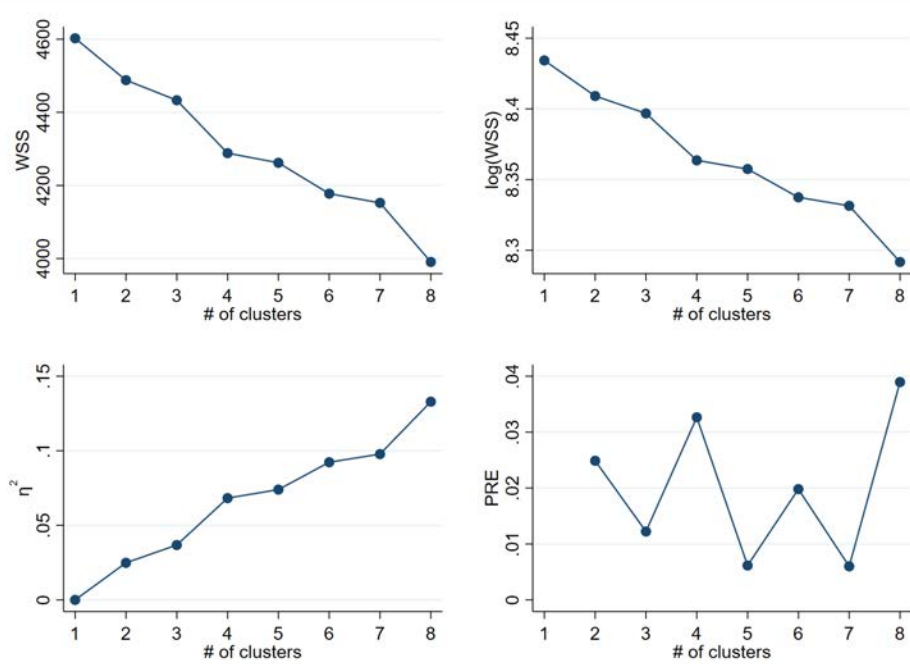
Panel A: Elbow method
