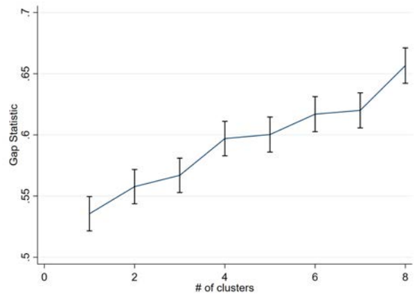
Panel C: Gap statistic
