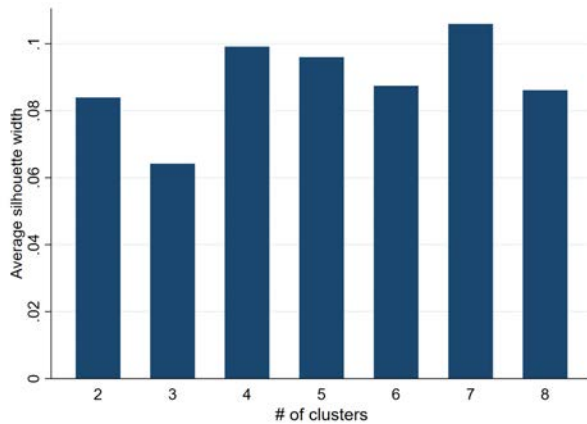
Panel B: Silhouette width
